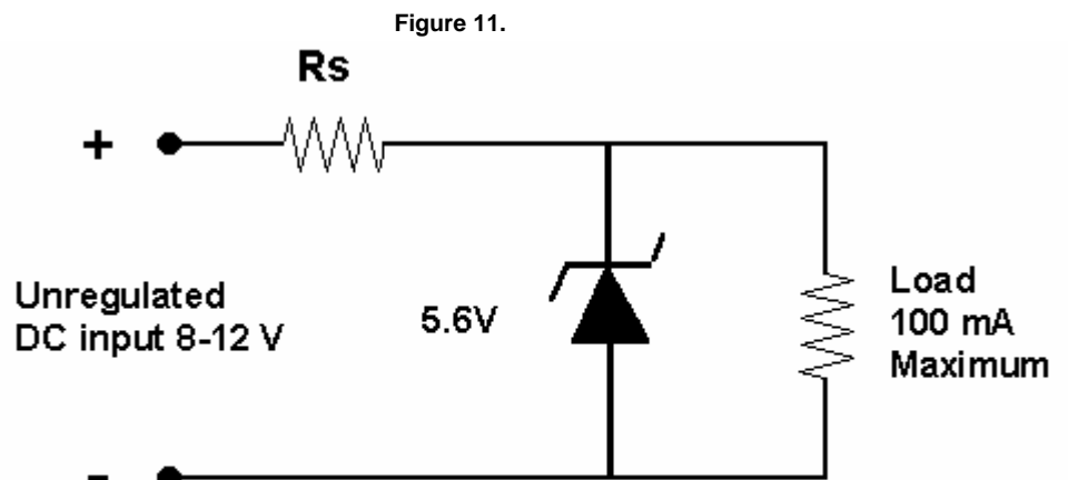
Zener diode used as shunt voltage regulator
