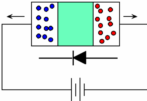
Reverse bias
